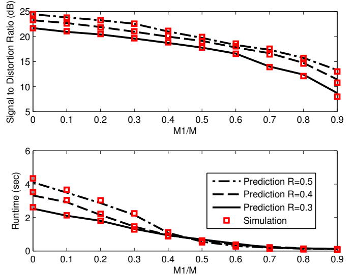
Figure 5: Top: Numerical verification of the prediction for SDR (15) of Noisy-Sudocodes with AMP in Part 2. Bottom: Numerical verification of the prediction for runtime of Noisy-Sudocodes with AMP in Part 2. ( N = 20,000 , s = 0.01 , and input SNR = 10 dB).
