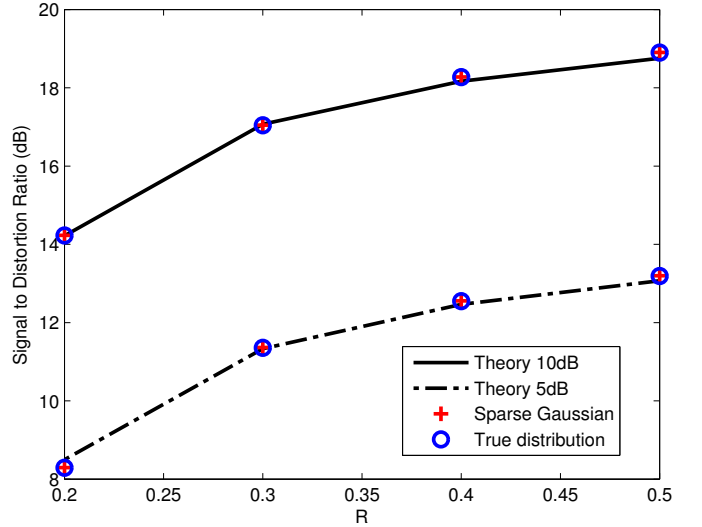
Figure 3: Numerical verification of sparse Gaussian approximation to the prior of \mathbf{x}_{\mathcal{T}} (8). ( N = 20,000 , s = 0.01 , and input SNR = 5 or 10 dB).
